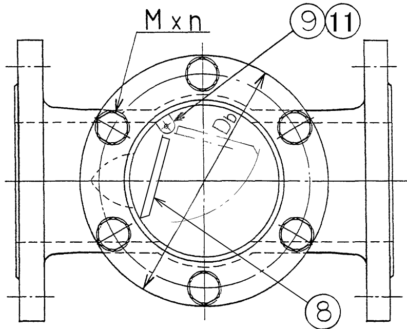
VIEW X-X
